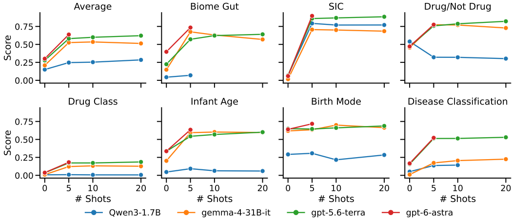
Figure 3: Few-shot classification results. 10-shot and 20-shot results are missing for some open model tasks due to them exceeding the context length. These results are missing for GPT-6-Astra for cost reasons. We choose to report five-shot results in the main text as they provide a reasonable trade-off between performance, coverage, and cost.
