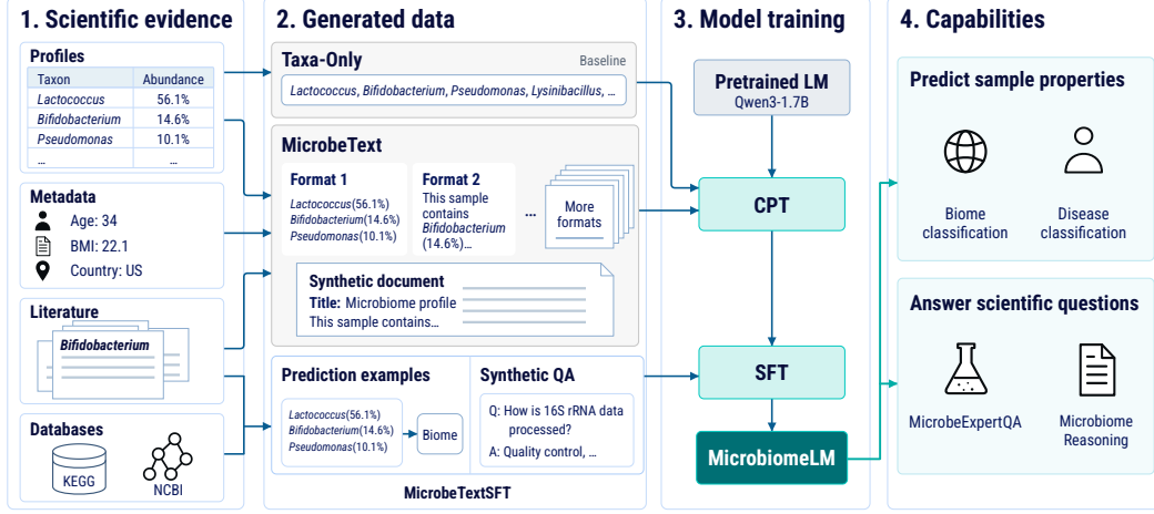
Figure 1: Overview of our microbiome data-generation and model-training pipeline. 1. Sample profiles, study metadata, literature, and biological databases provide scientific evidence. 2. Taxa-Only represents profiles as ranked taxon-name sequences. MicrobeText transforms study data and literature-derived facts into diverse profile formats and synthetic documents. MicrobeTextSFT mixes classification examples with synthetic question-answer pairs. 3. An existing language model is adapted through continued pretraining (CPT) and supervised finetuning (SFT). 4. Models are evaluated on sample-property prediction and scientific question answering.
