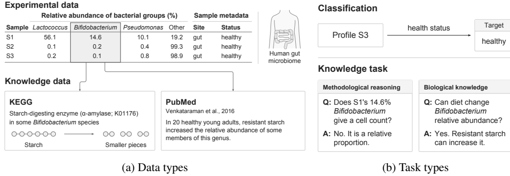
Figure 2: Microbiome data and task types. (a) Microbial names connect abundance profiles to structured biological annotations and scientific literature. (b) Classification tasks infer sample attributes from abundance profiles, while knowledge tasks assess biological understanding and methodological reasoning through scientific question answering.
